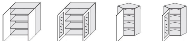
W4/90 900/960/325 W4S/90 900/960/325 W4/10/60 600/960/600 W4S/10/60 600/960/600
