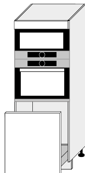
D5AE/60/154* 600/1540/565
