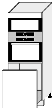
D5AM/60/154 600/1540/565
