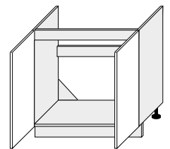
D8Z/80 800/820/500
