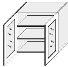
W3S/80 800/720/325* 800/720/300**
