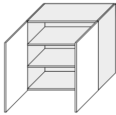
W3/80 800/720/325* 800/720/300**
