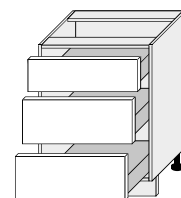
D3E/60* 600/820/500
