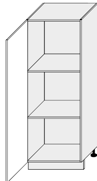
D5D/60/154 600/1540/565
